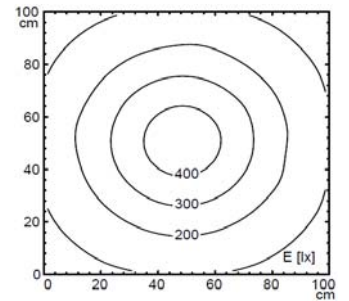
Light measurement
